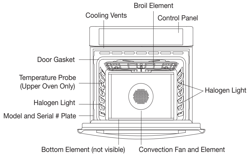
Cooling Vents
